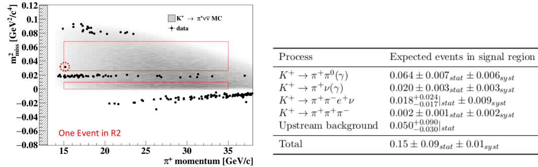
Figure 3: Left panel: m_{\text{miss}}^2 as function of \pi^+ momentum. Data passing the K^+ \rightarrow \pi^+ \nu \bar{\nu} selection appear in the red boxes. The grey area is the distribution of events for K^+ \rightarrow \pi^+ \nu \bar{\nu} from MC. One event is observed in the R2 signal box. Right panel: Table of expected background contributions in signal regions.
