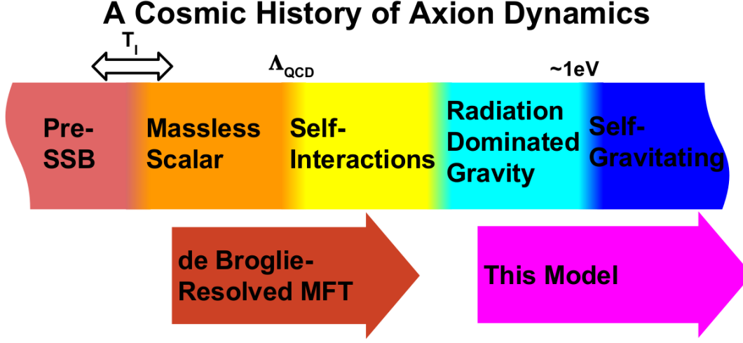
Figure 1: Cosmological history of QCD axion dynamics. Early time and high temperature conditions are to the left, running to late time and cold conditions to the right. It is a typical feature of QCD axion theories that the ordering of inflation ( T_I ) and the spontaneous symmetry breaking (SSB) of the axion's parent scalar is uncertain. Some time later, the QCD phase transition ( \Lambda_{\text{QCD}} ) provides the axion field with a mass and consequently its status as a DM candidate. Further cosmic expansion brings the gravity of fluctuations into dominance for the axion, marginalizing the effectiveness of mean field models (MFTs) and highlights the model presented here.
