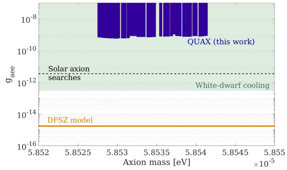
Figure 3: Excluded values of the g_{aee} coupling (blue area) compared to its theoretical prediction for the DFSZ axion model (orange line) and a DM density of 0.45 \text{ GeV}/\text{cm}^3 . The green shaded area is excluded by white dwarf cooling, while the black dashed line is the best upper limit obtained with solar axion searches relying on the axio-electric effect (See ref. [2] for details).
